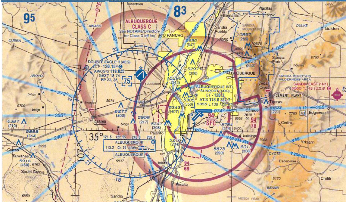
Figure 1.3 Albuquerque Sectional Chart
