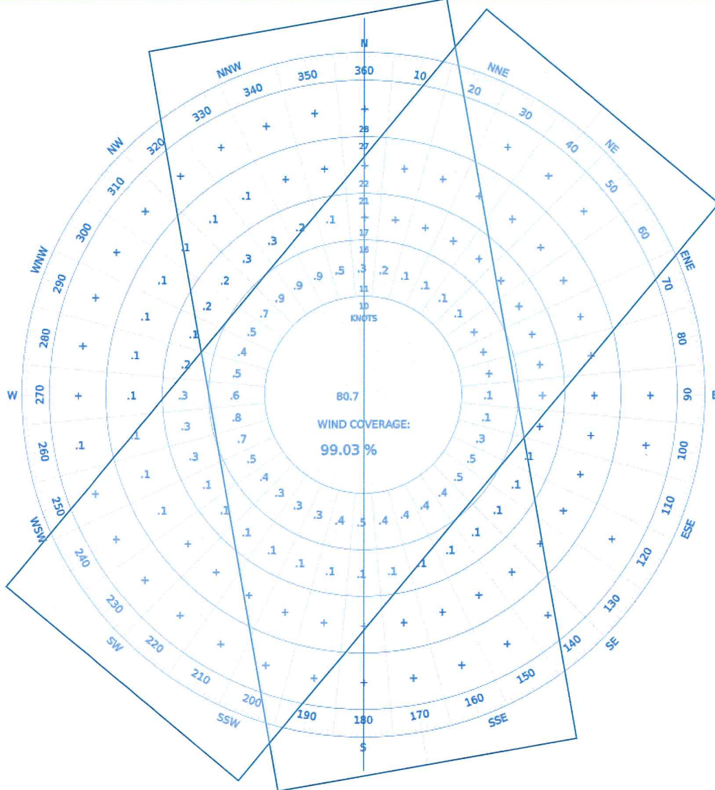
Figure 3.4 Wind Rose
