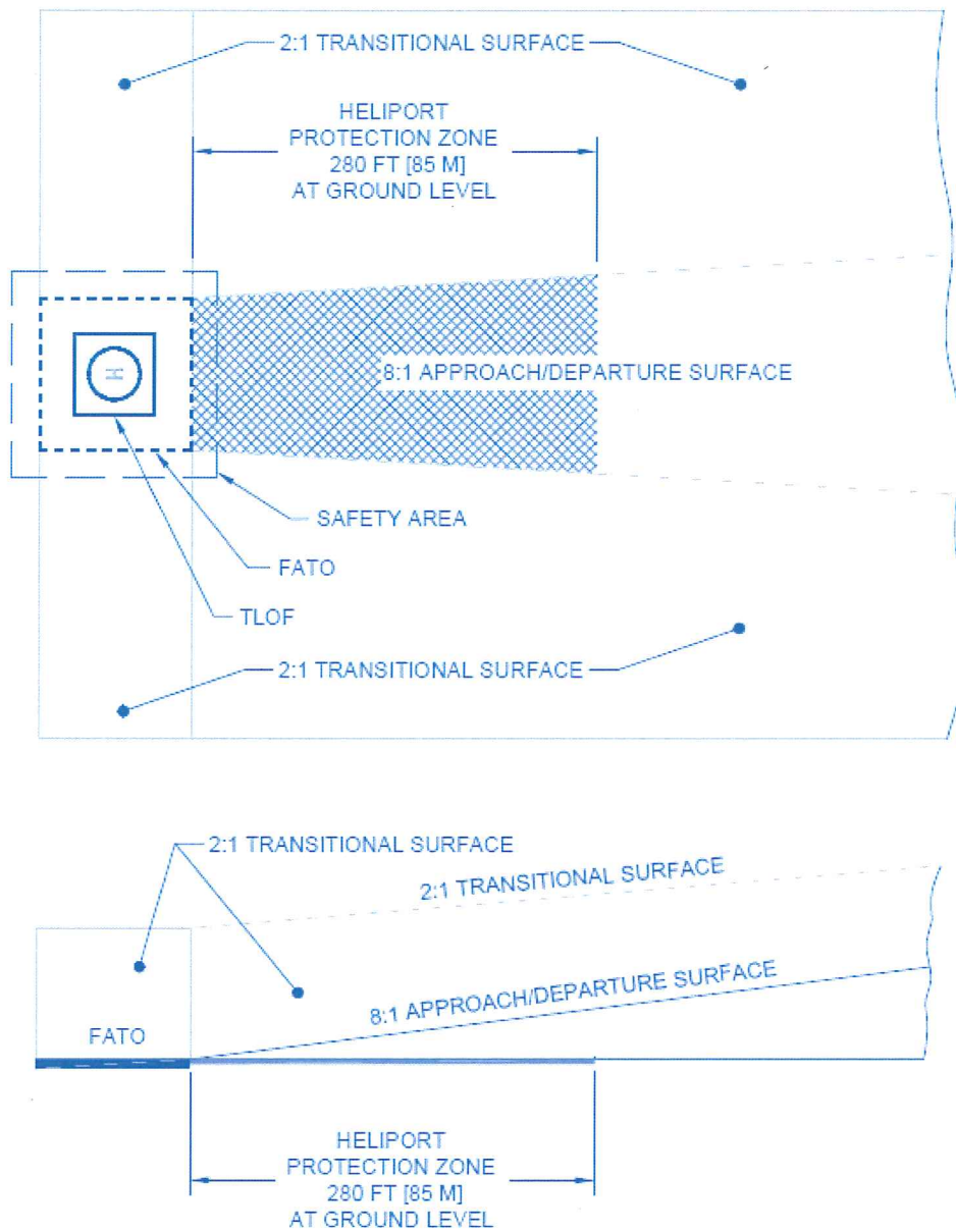
Figure 3.10 FAA Recommended Heliport Protection Zone
