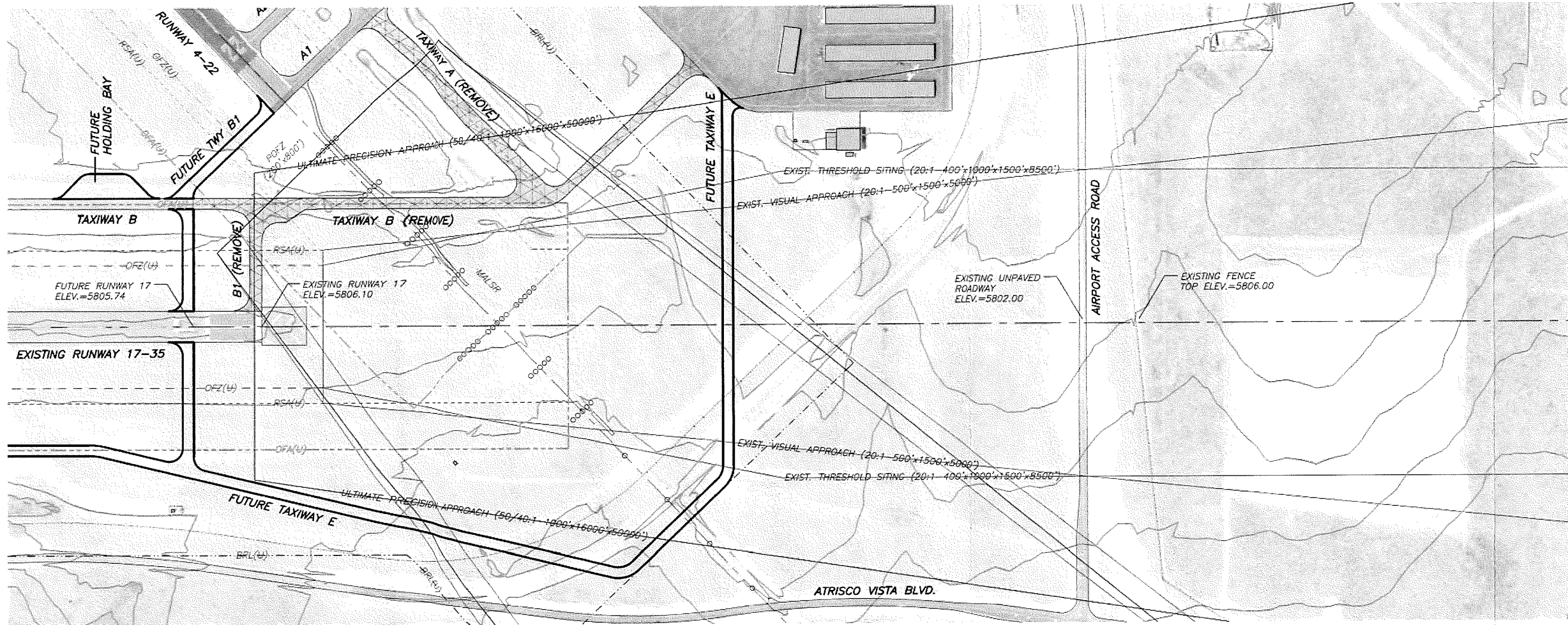
RUNWAY 17 - PLAN
