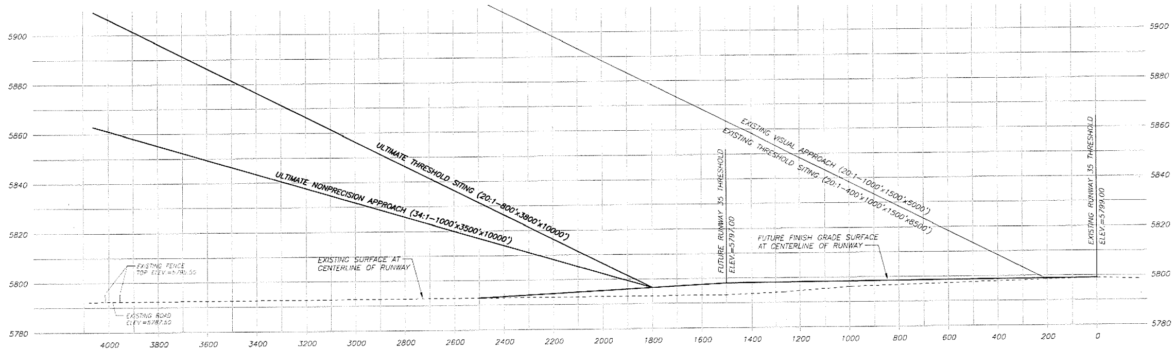
RUNWAY 35 - PROFILE
