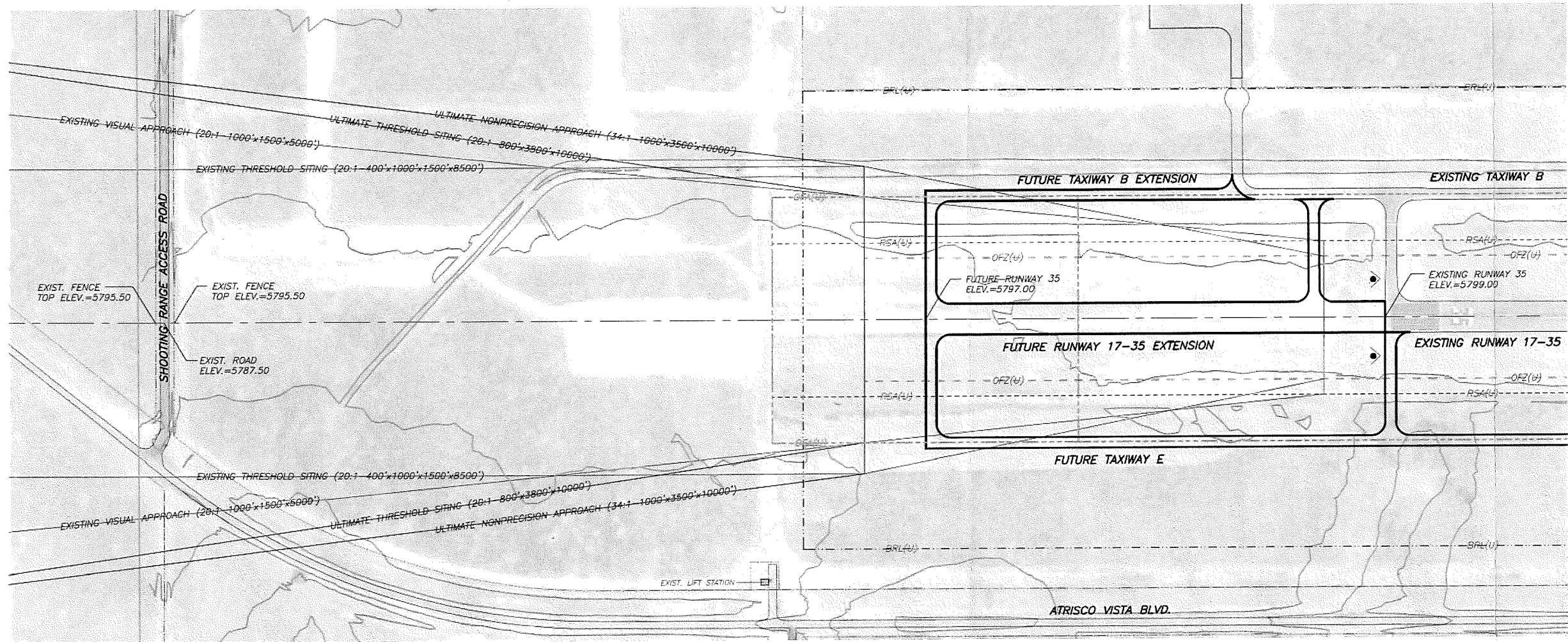
RUNWAY 35 - PLAN
