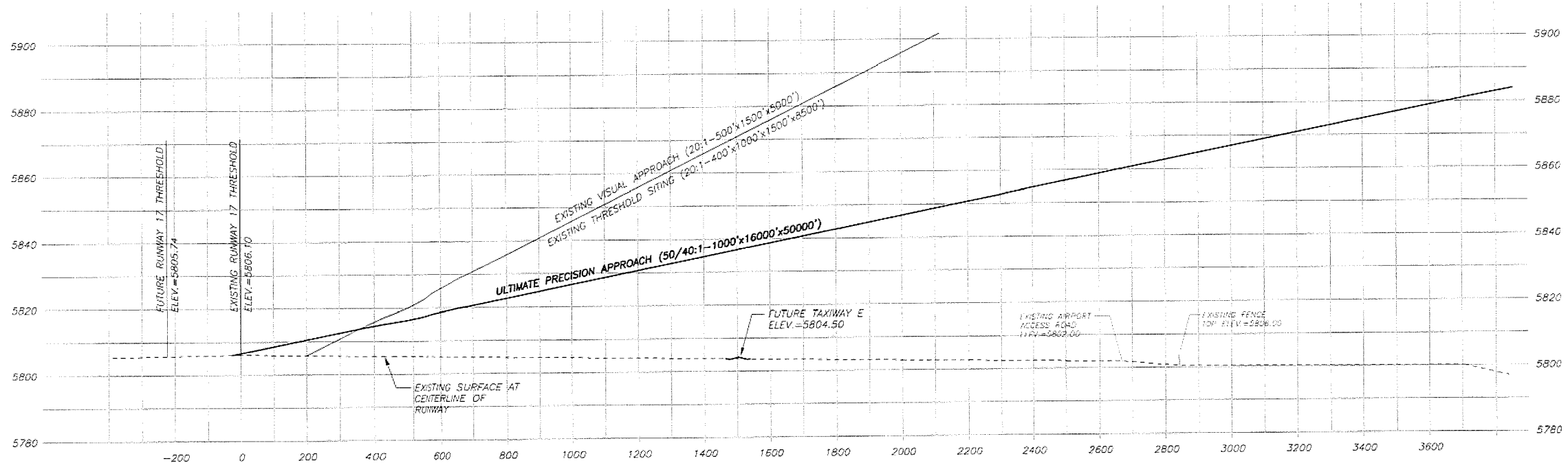
RUNWAY 17 - PROFILE
