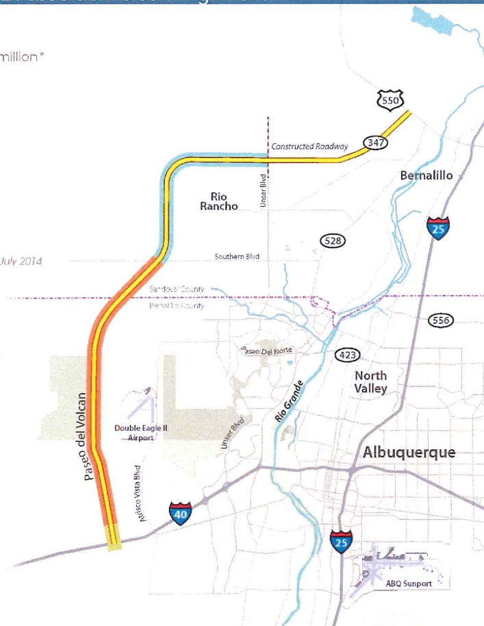
Figure 2.2 Paseo del Volcan Alignment
