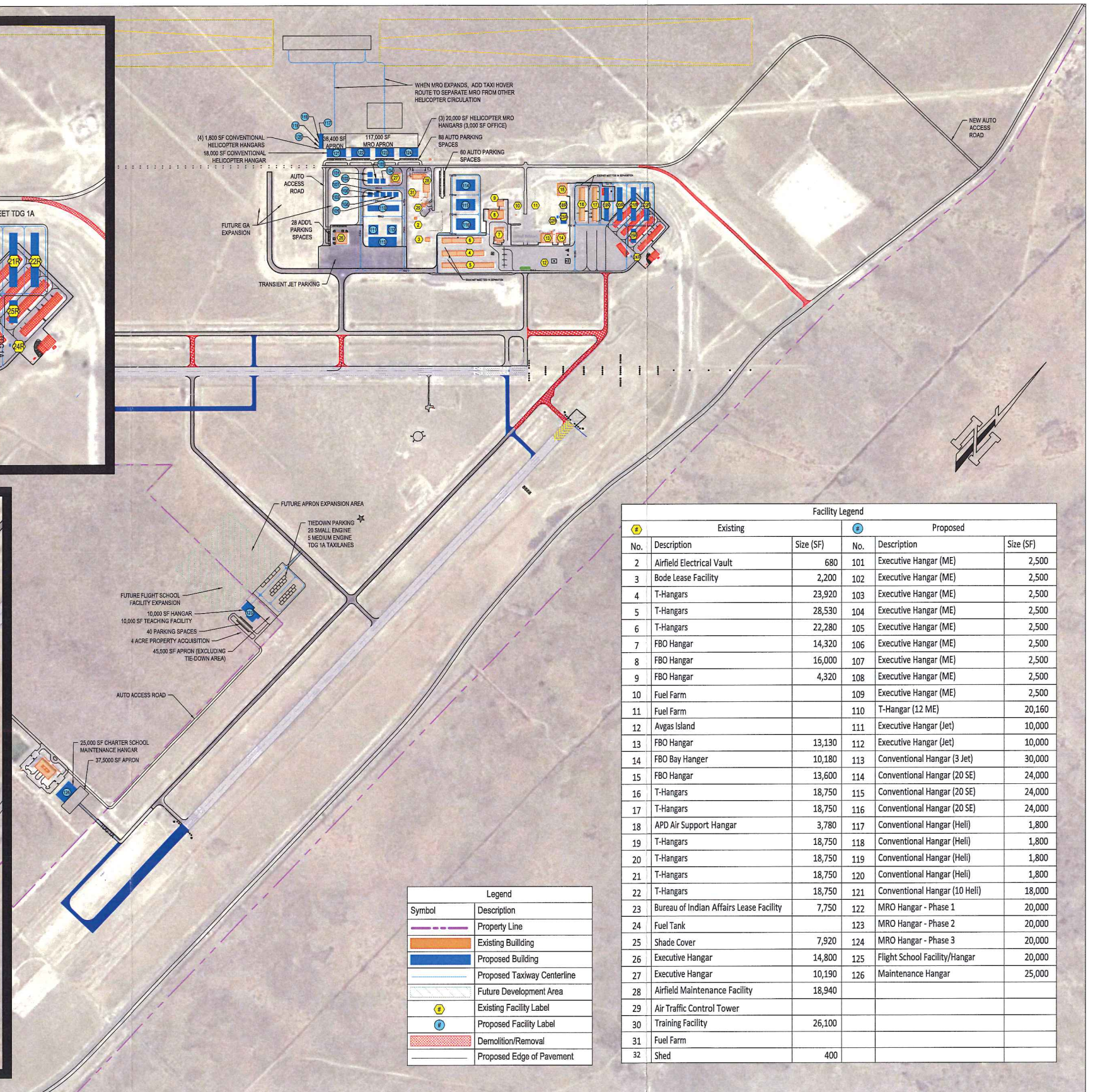
Double Eagle II Airport Master Plan
