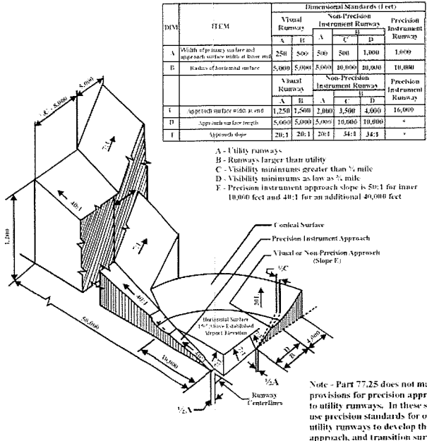
PART 77 AIRSPACE - ISOMETRIC VIEW
