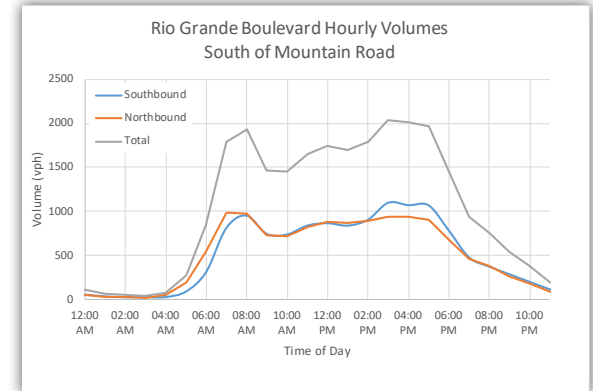
Figure 3-2: Hourly Traffic Volumes on Rio Grande Boulevard
