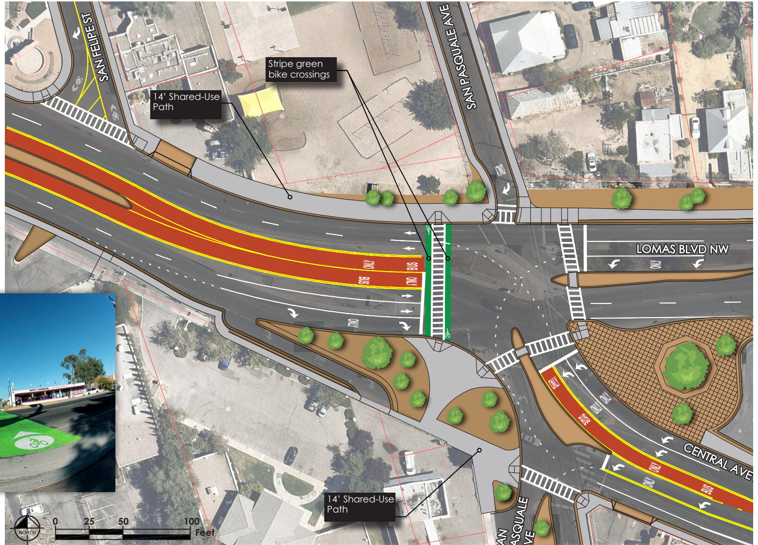
Figure 4-11: Central Avenue Crossing Improvement
