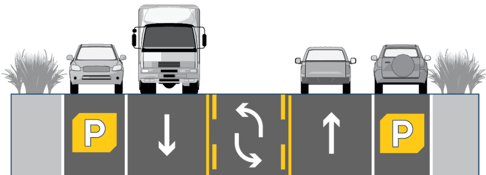
③ Three-lane road with center turn lane and on-street parking.
