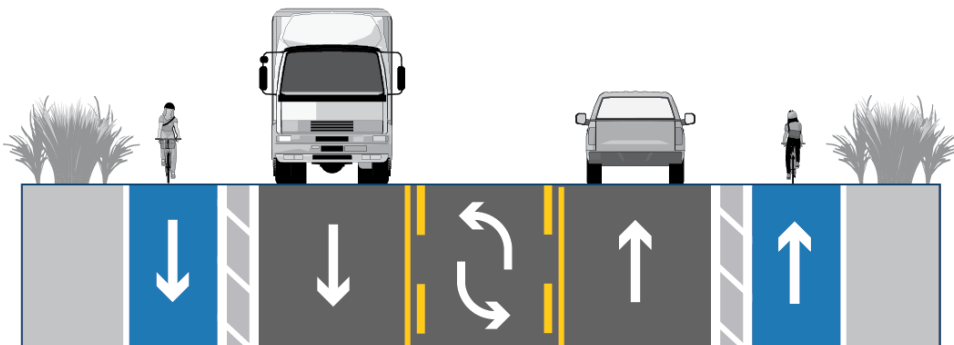
② Three-lane road with center turn lane and buffered bike lanes.
