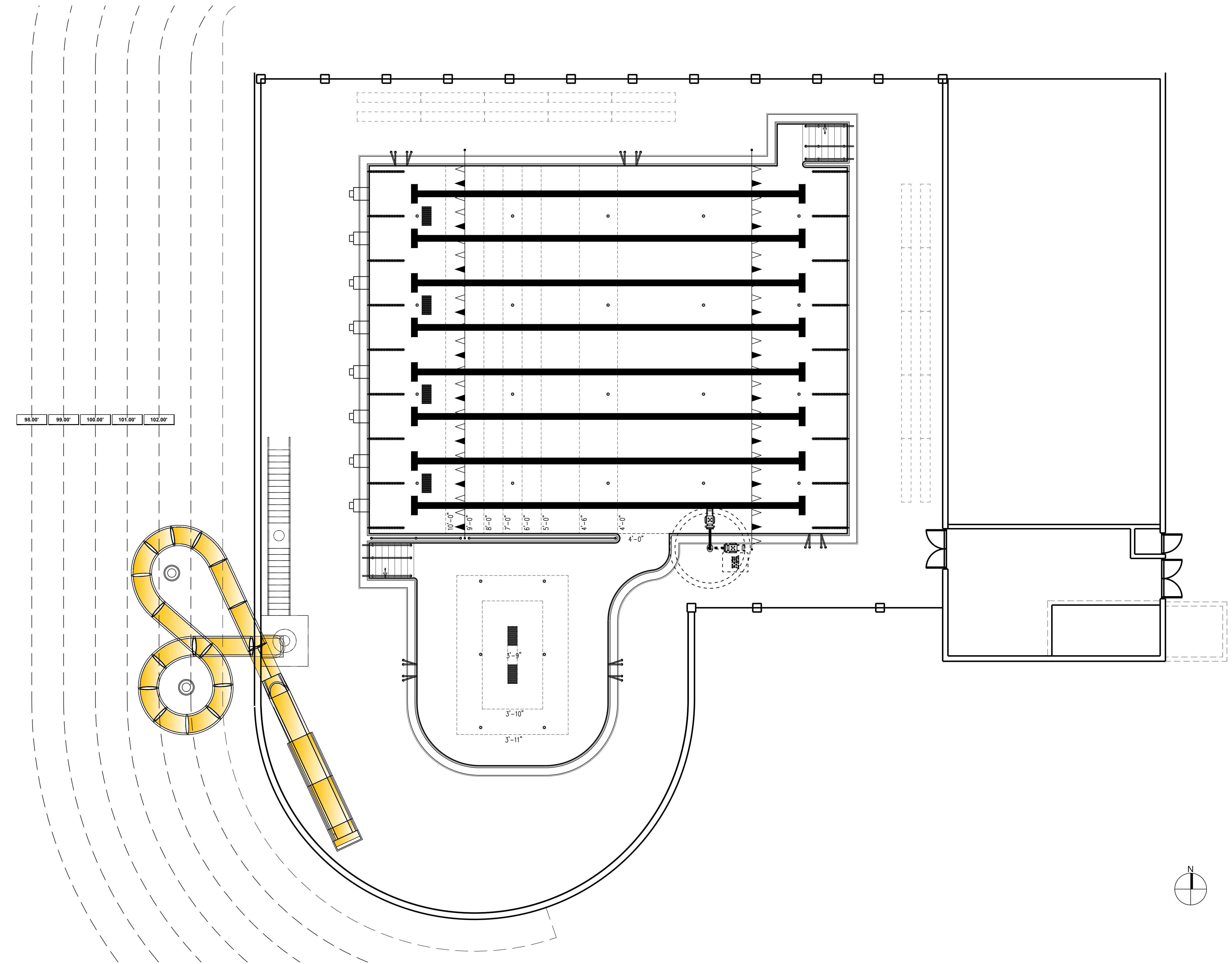
LEISURE POOL FLOOR PLAN
